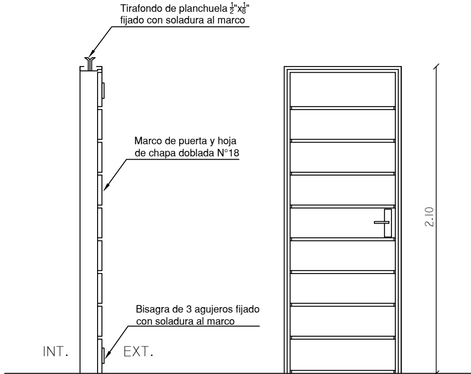
CORTE VERTICAL
