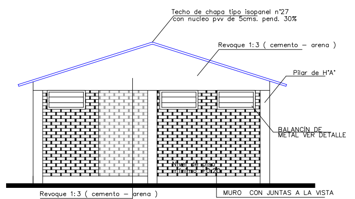
FACHADA PRINCIPAL ESCALA.....1:100
