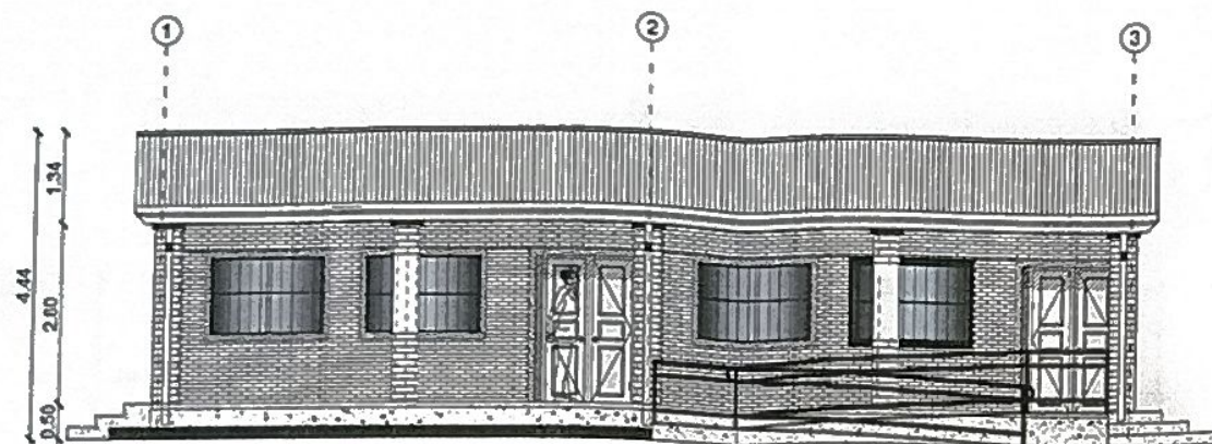
FACHADA PRINCIPAL
